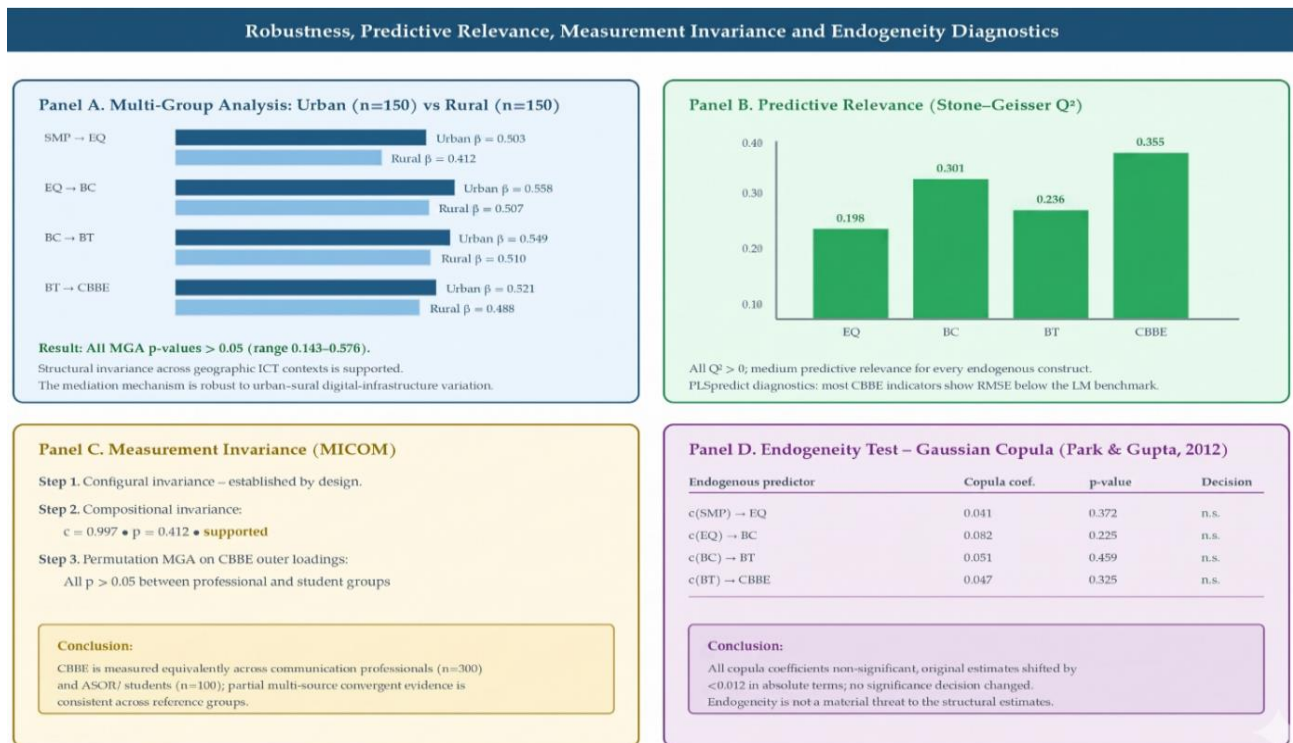
Fig. 2. Robustness, measurement-invariance and endogeneity-assessment summary.
